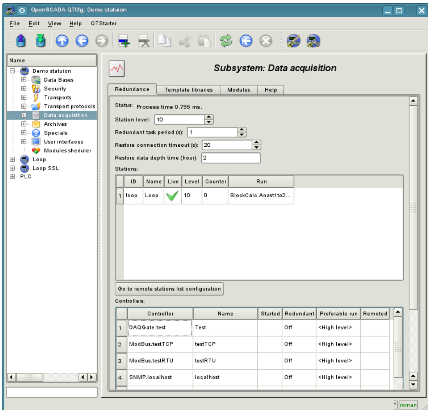
Fig. 4.5b. Tab "Redundance" tab of subsystem "Data acquisition".
