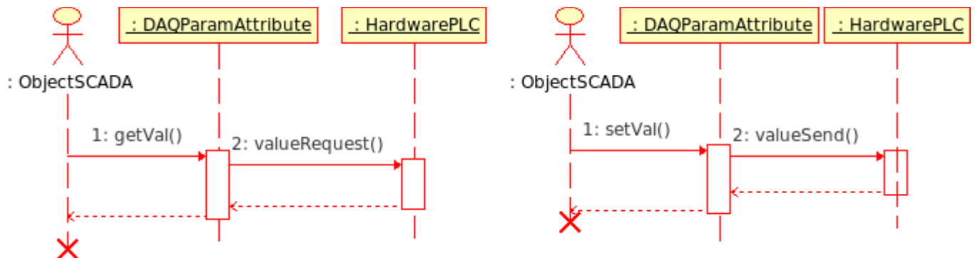
Fig. 2. Diagram of the sequence of interaction with the synchronous requests.
