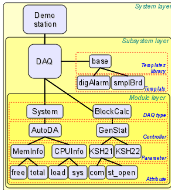
Fig. 1. The subsystem's "Data acquisition" scheme.
