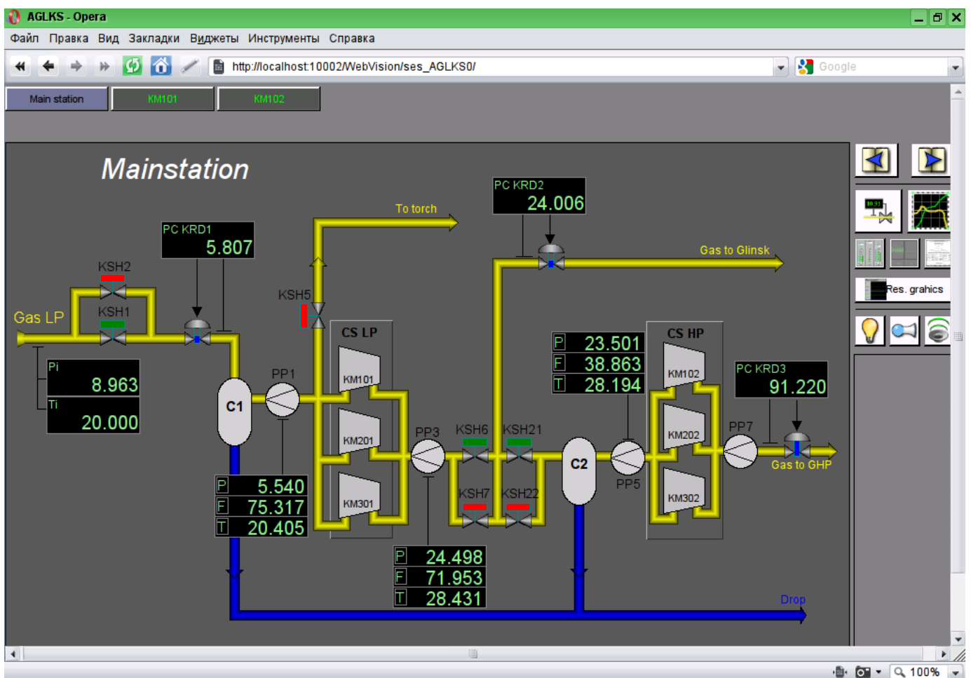
Fig.3. The main execution window.
