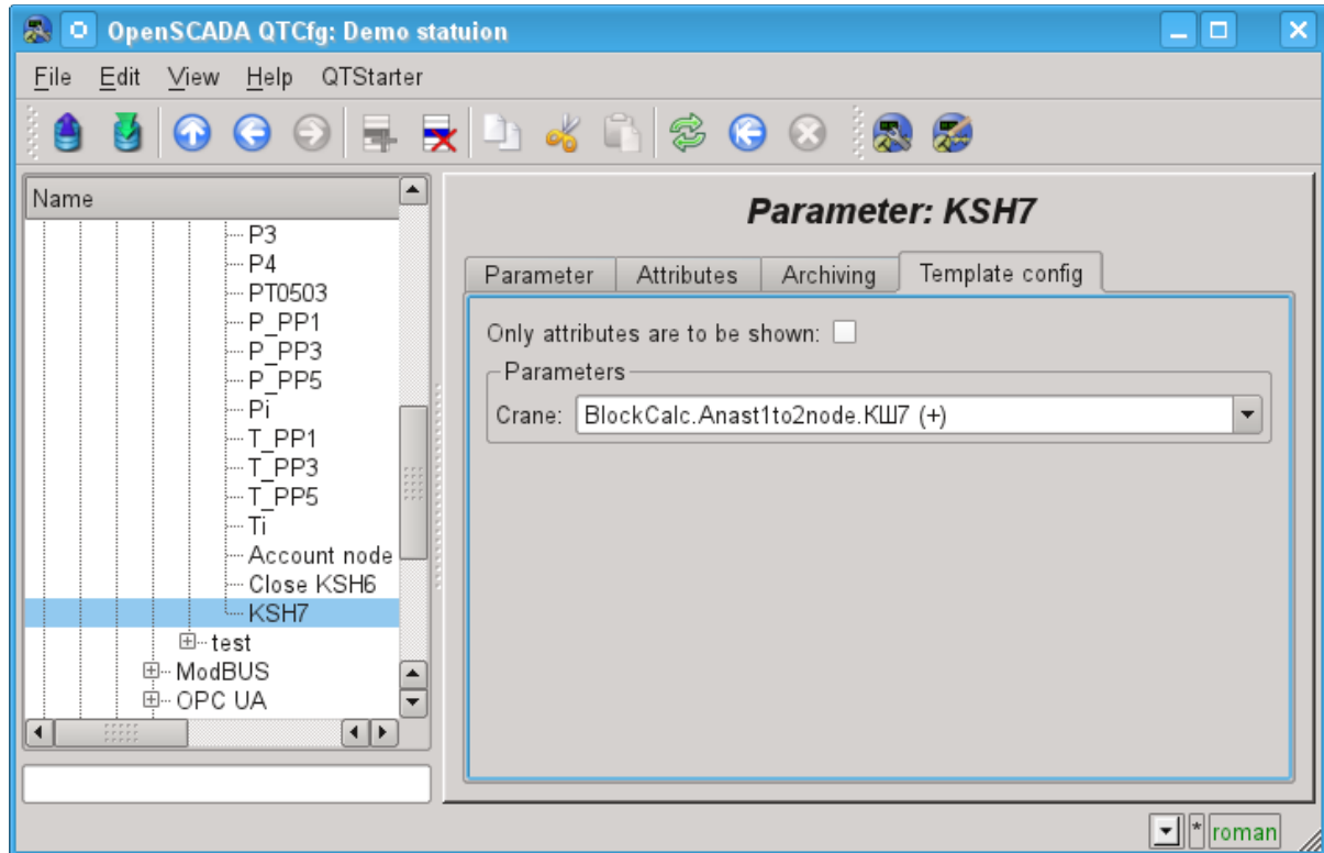
Fig.3. Configuration tab of the template of parameter.
