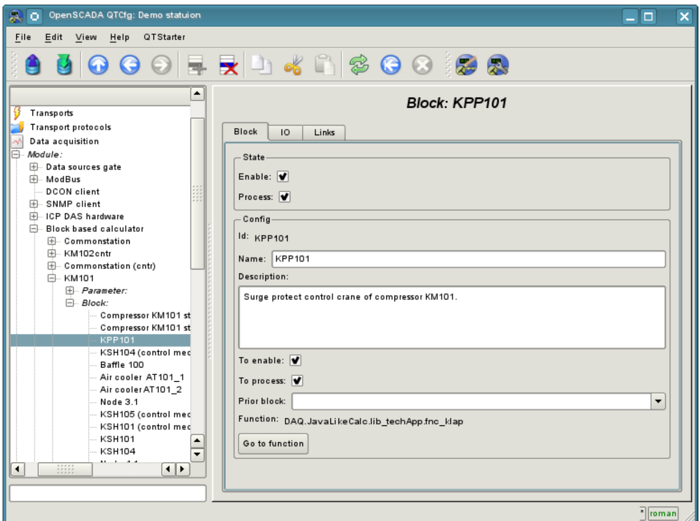
Fig. 4. Configuration tab of the block scheme.
